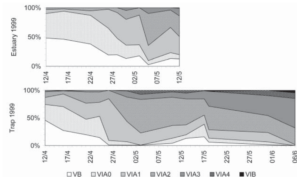
Figure 4 Seasonal changes in pigment stages for samples collected on the trapping ladder and in the estuary in 1999.
